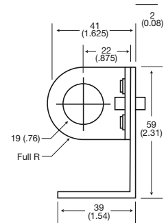
Adjustable Mounting Bracket
